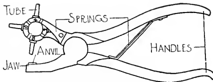
FIG. 100. BELT PUNCH.
